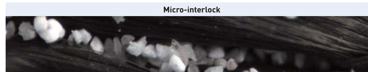
Micro-interlock Synonym for friction/adhesion: microscopic interlock of soil particles with grid surface. 20-fold magnification: rough surface texture of Fortrac, pictured here with 0.1-0.3 mm sand particles which achieve interlock at microscopic level and increase friction.
