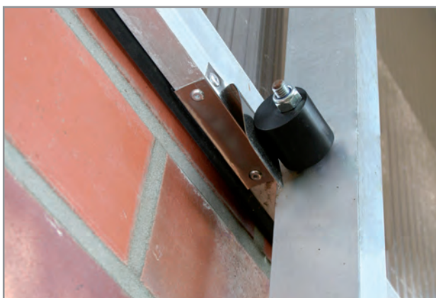
Close-up of clamping system
