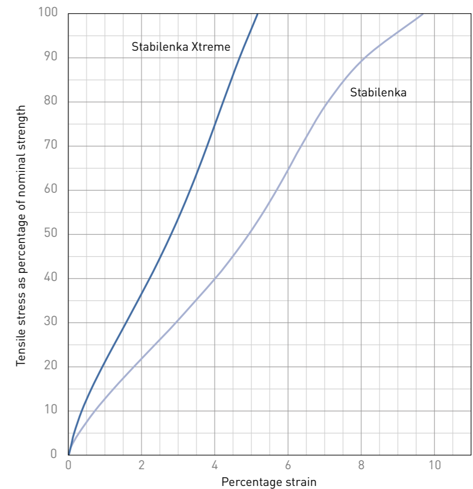
Specimen short term tensile stress-strain curves
